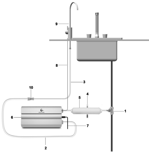
(A) Installation with Smart Faucet
